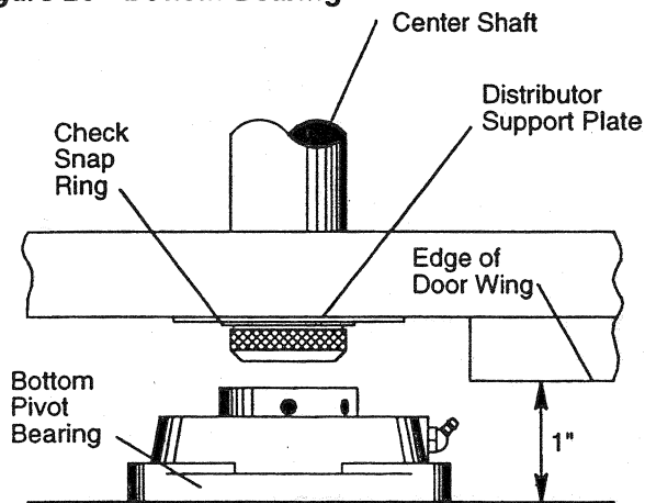
Figure 28 - Bottom Bearing
