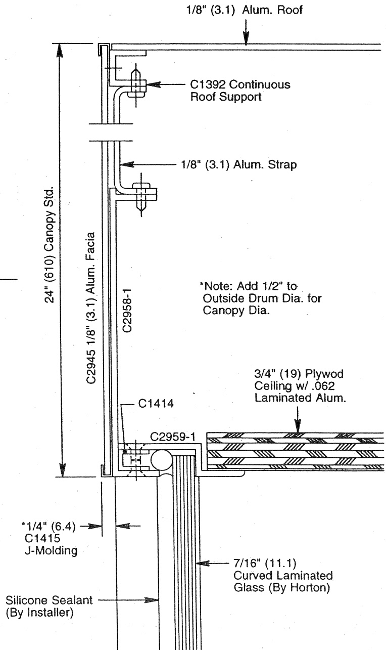
Figure 20 - Round Revolving Door Canopy
