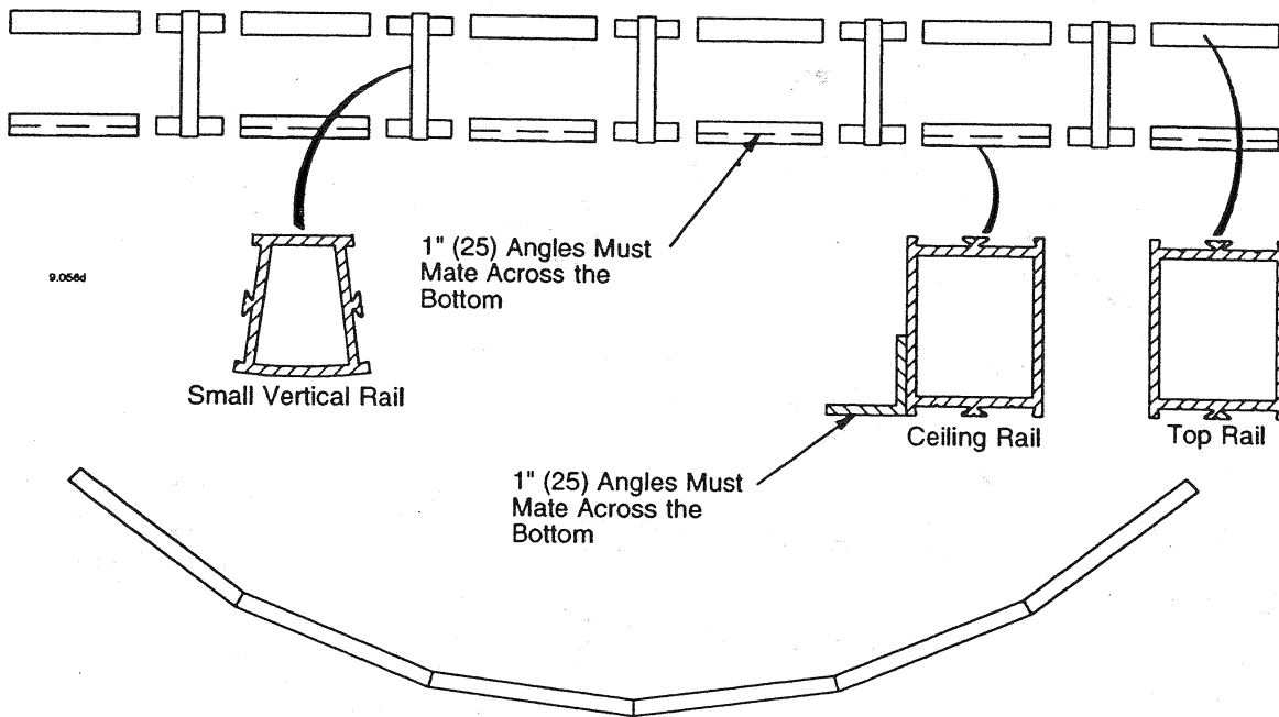
Figure 8- Center Canopy Section Assembly (Segmented Canopy)
