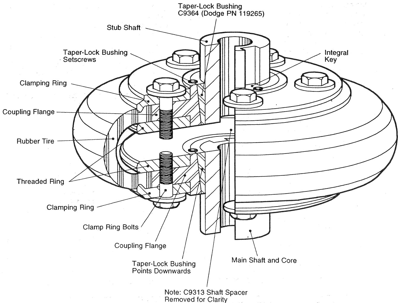
Figure 31- C9373-1 Coupling Assembly
