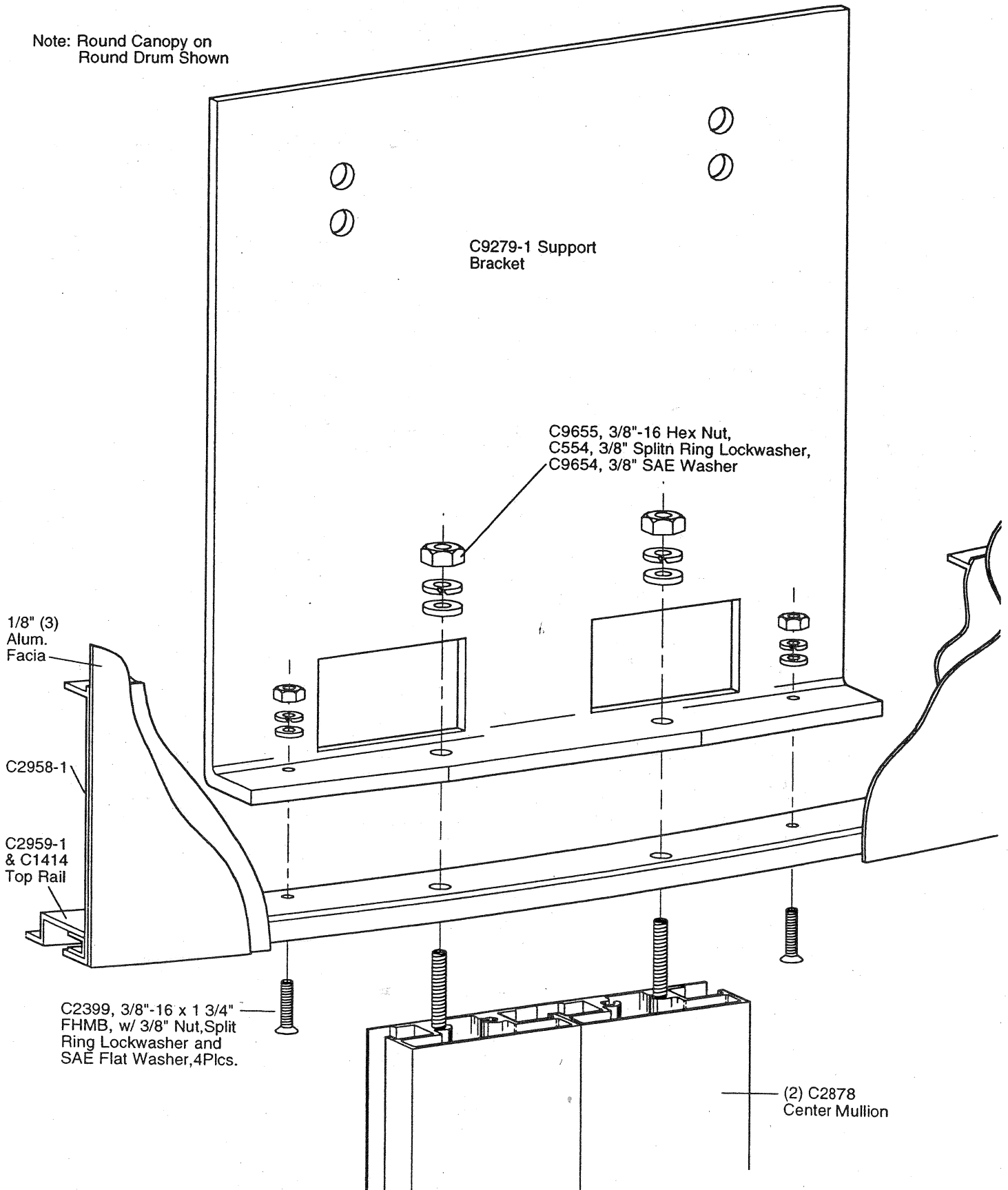
Figure 18 - Gear Train Support Bracket Installation (Round Canopy)
