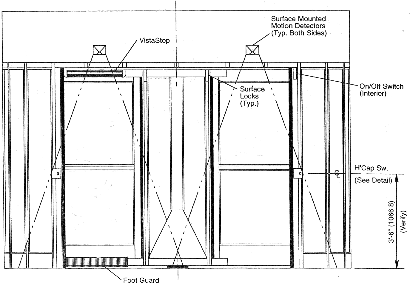
Figure 47 - Elevation of 4 Wing Grand Revolving Door
