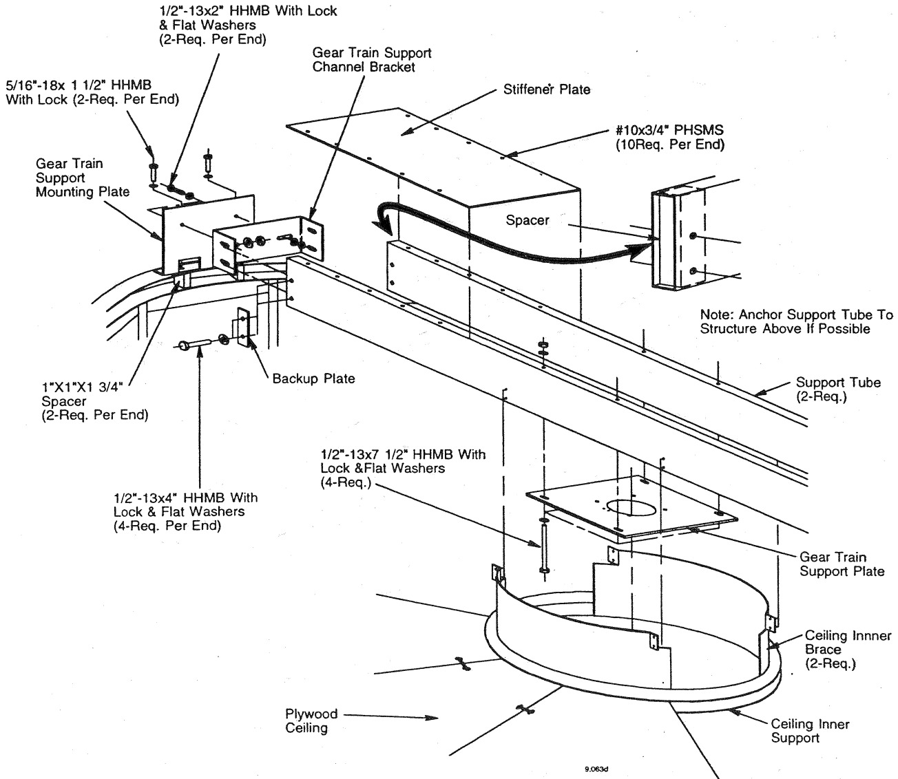
Figure 22 - Gear Train Support (Round Canopy)
