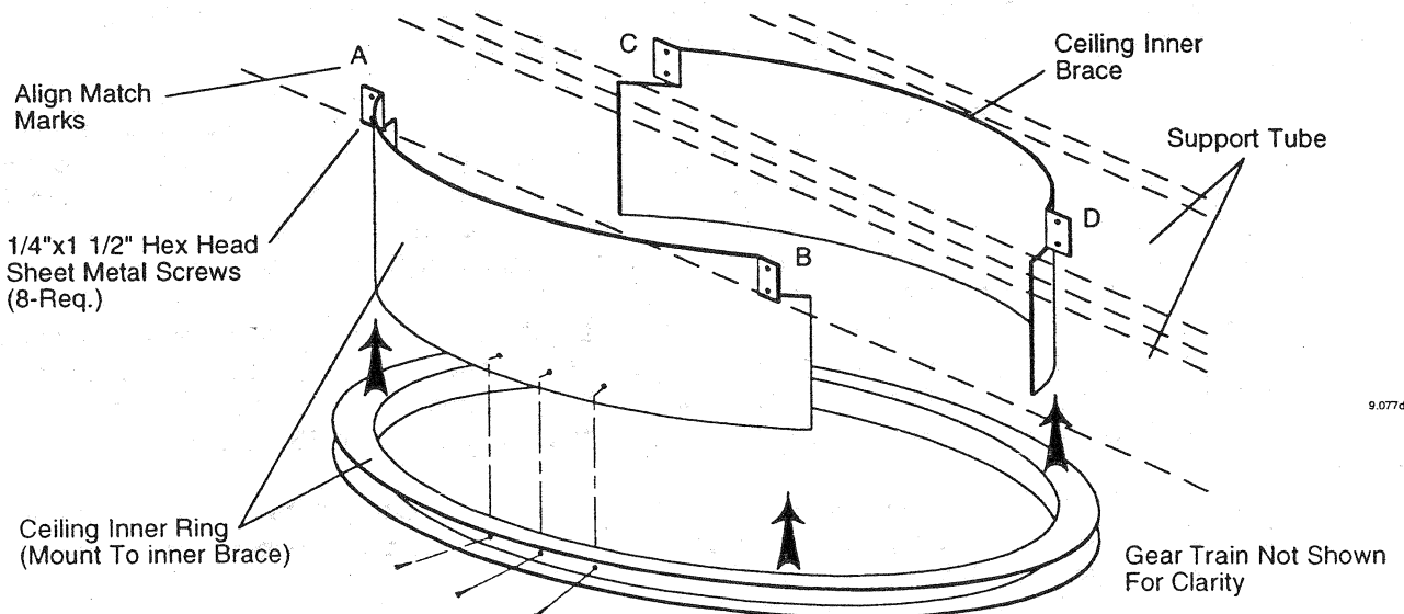
Figure 34 - Ceiling Supports
