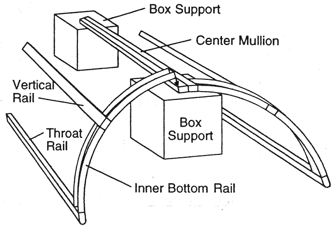
Figure 16 - Vertical Rail Assembly
