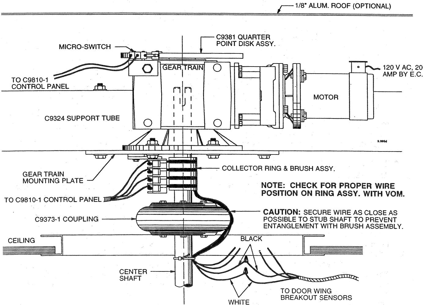
Figure 46 - Wiring Switches
