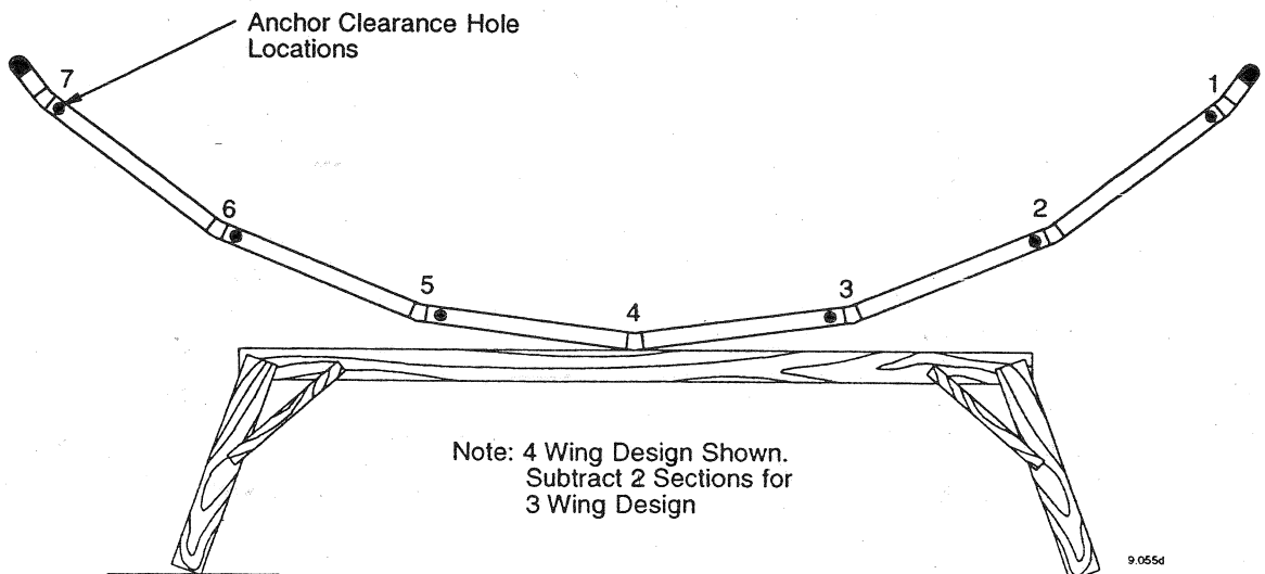
Figure 4 - Drum Assembly (Round Canopy)
