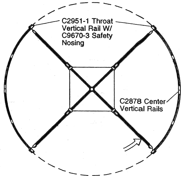
Figure 53 - Floor Plan of 4-Wing Round Grand Revolving Door
