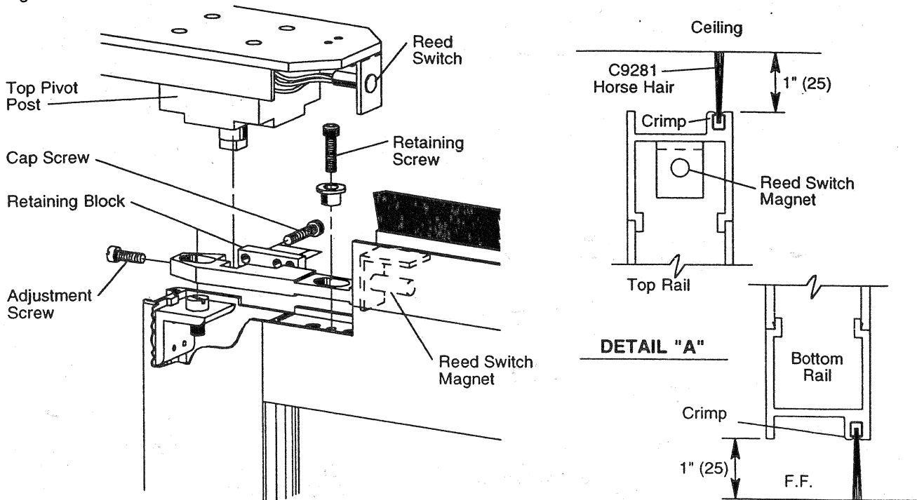
Figure 41 - Door Panels
