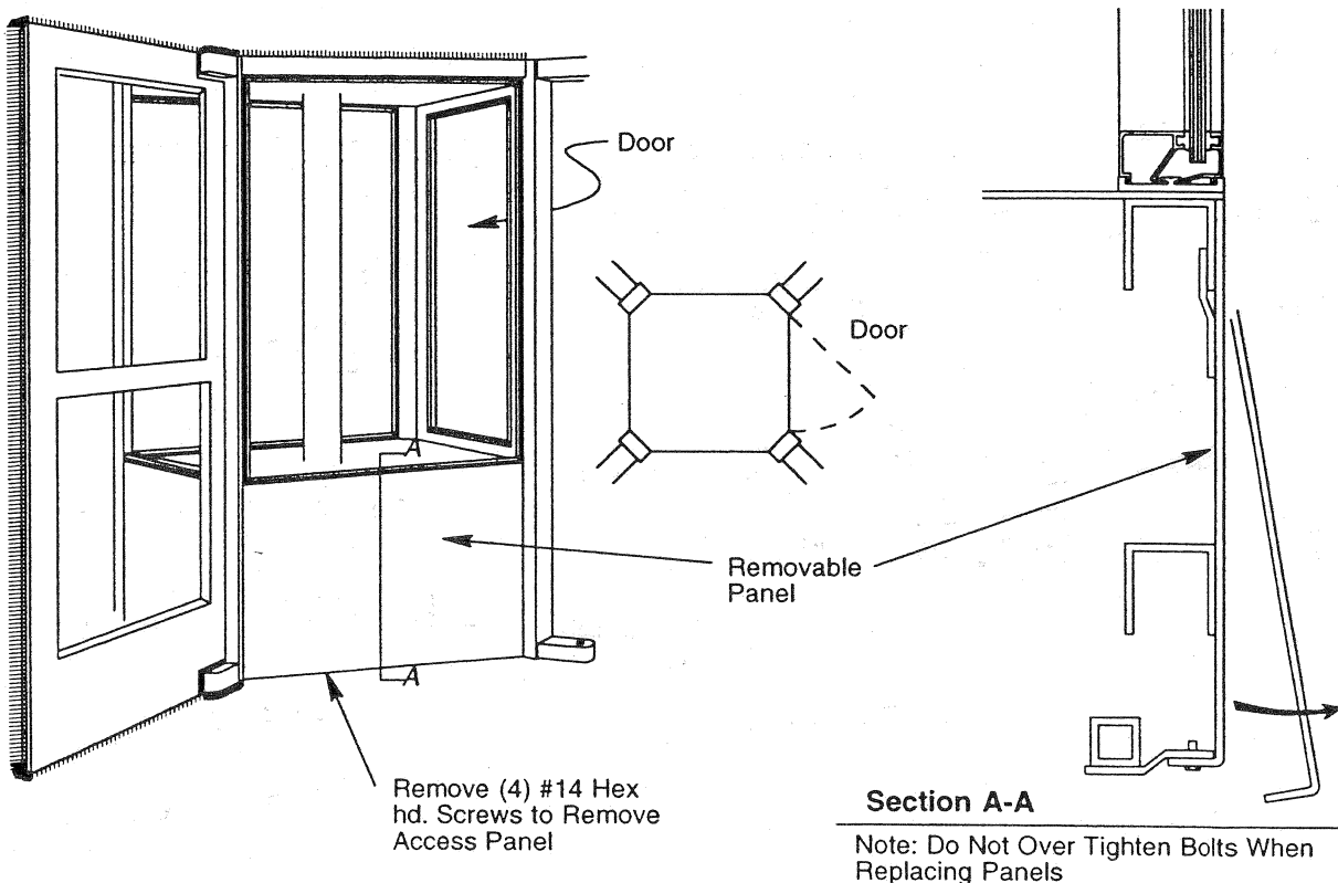
Figure 39 - Access Panel for Display Core
