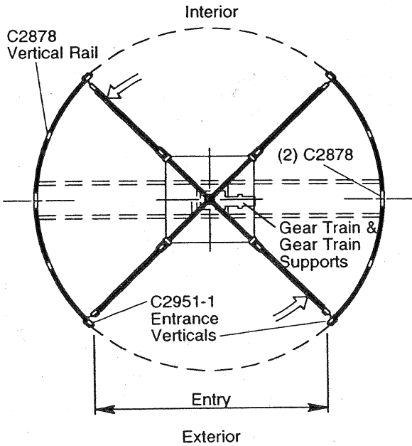
Figure 19 - Round Drum Orientation
