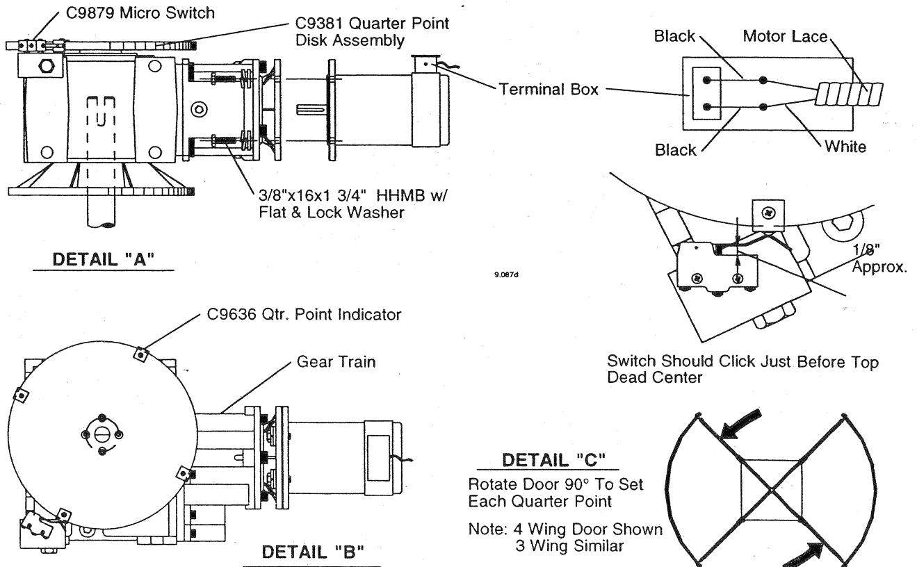
Figure 42 - Motor and Quarter Point Indicator
