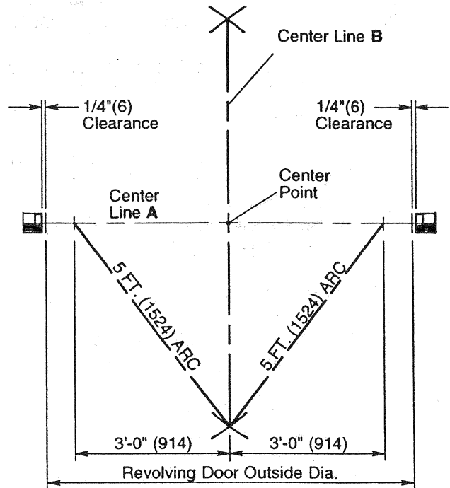
Figure 1 - Equal Arc Method
