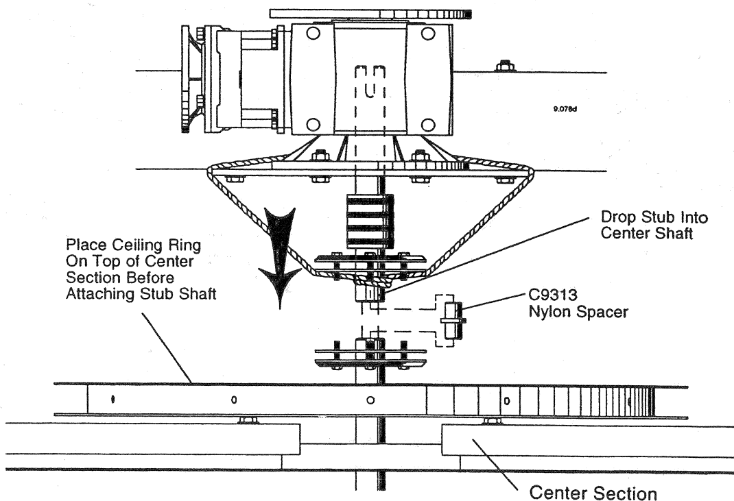
Figure 30 - Center Section Attachment
