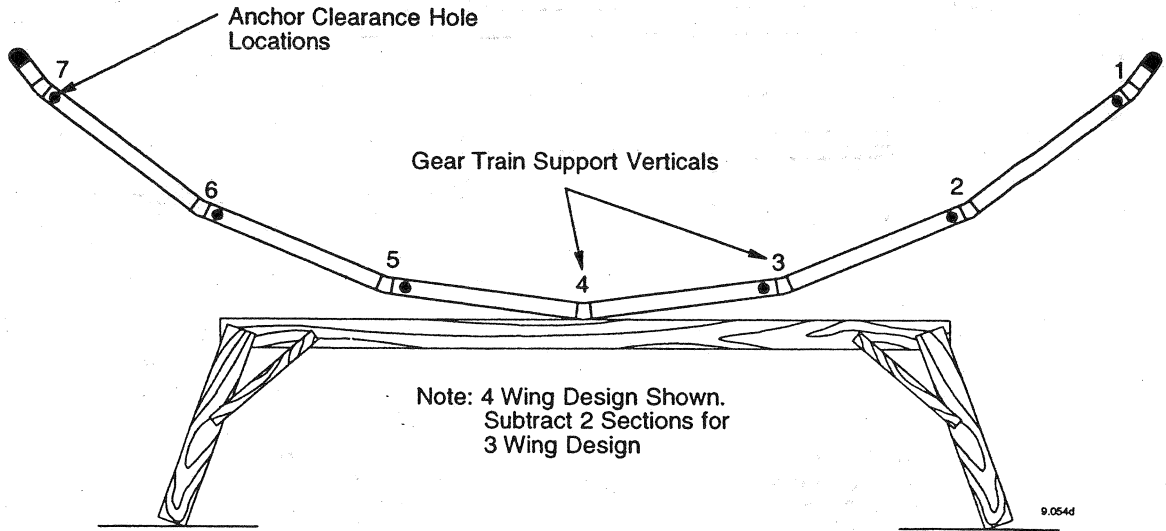
Figure 3 - Drum Assembly (Segmented Canopy)
