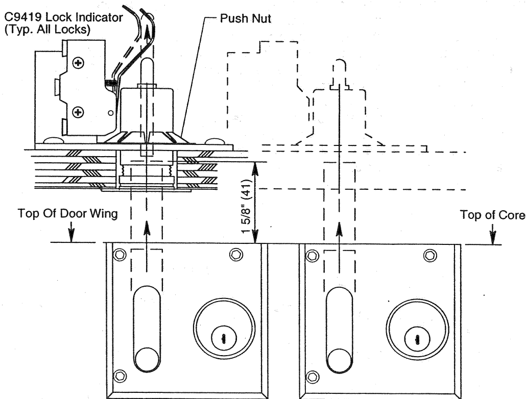
Figure 45 - Surface Locks and Microswitch
