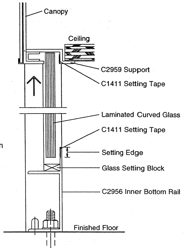
Figure 58 - Vertical Section
