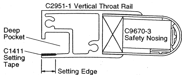
Figure 54 - Horizontal Section at Throat Rail
