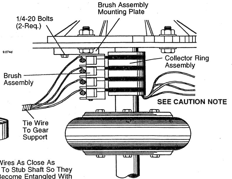
Figure 33 - Brush Assembly
