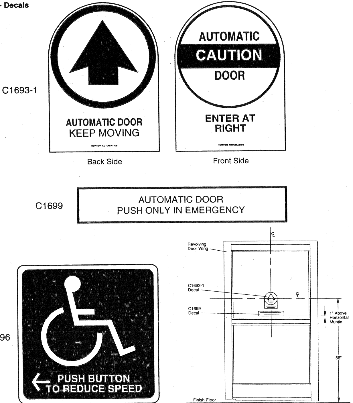
DOOR WING ELEVATION SHOWING DECAL LOCATION
