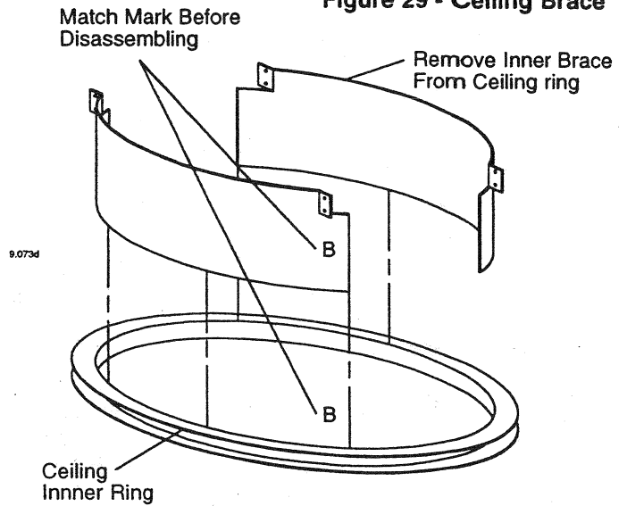
Figure 29 - Ceiling Brace
