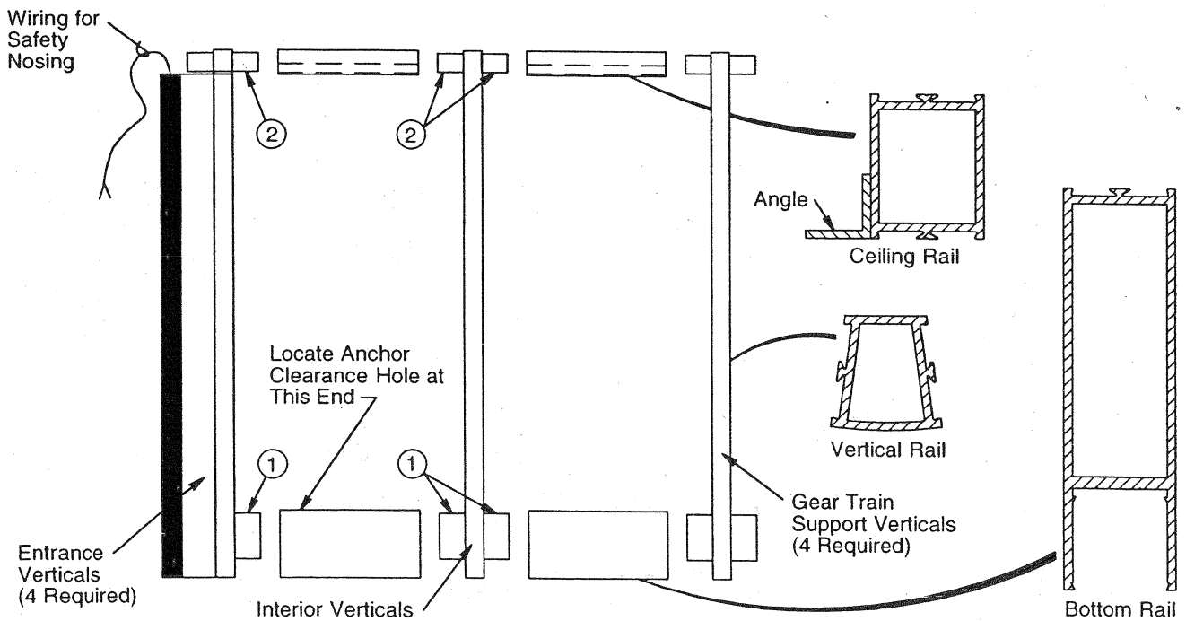
Figure 6 - Placement of Extrusions (Round Canopy) - View from Inside Door
