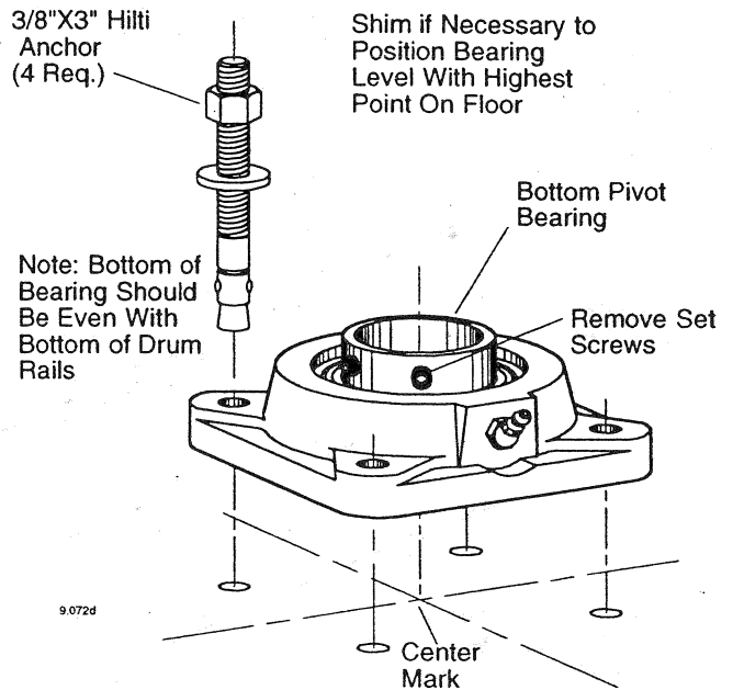
Figure 26 - Bottom Bearing
