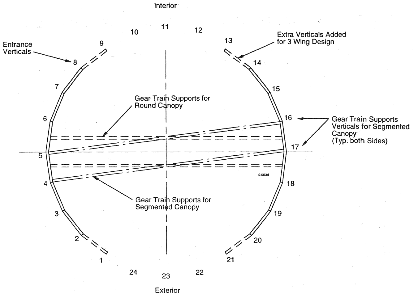
Figure 7 - Orientation of Drum Halves
