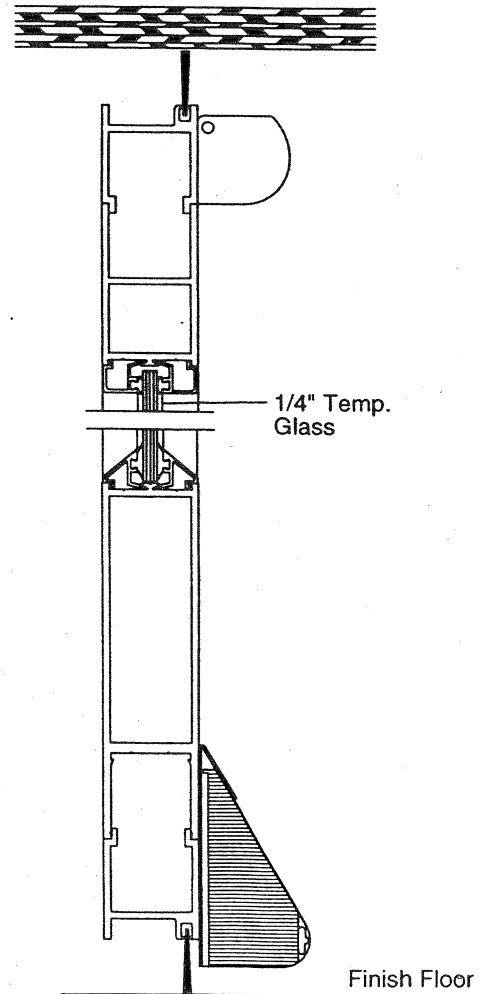
Figure 52 - Door Panel Section
