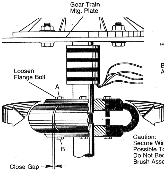
Figure 32 - Coupling
