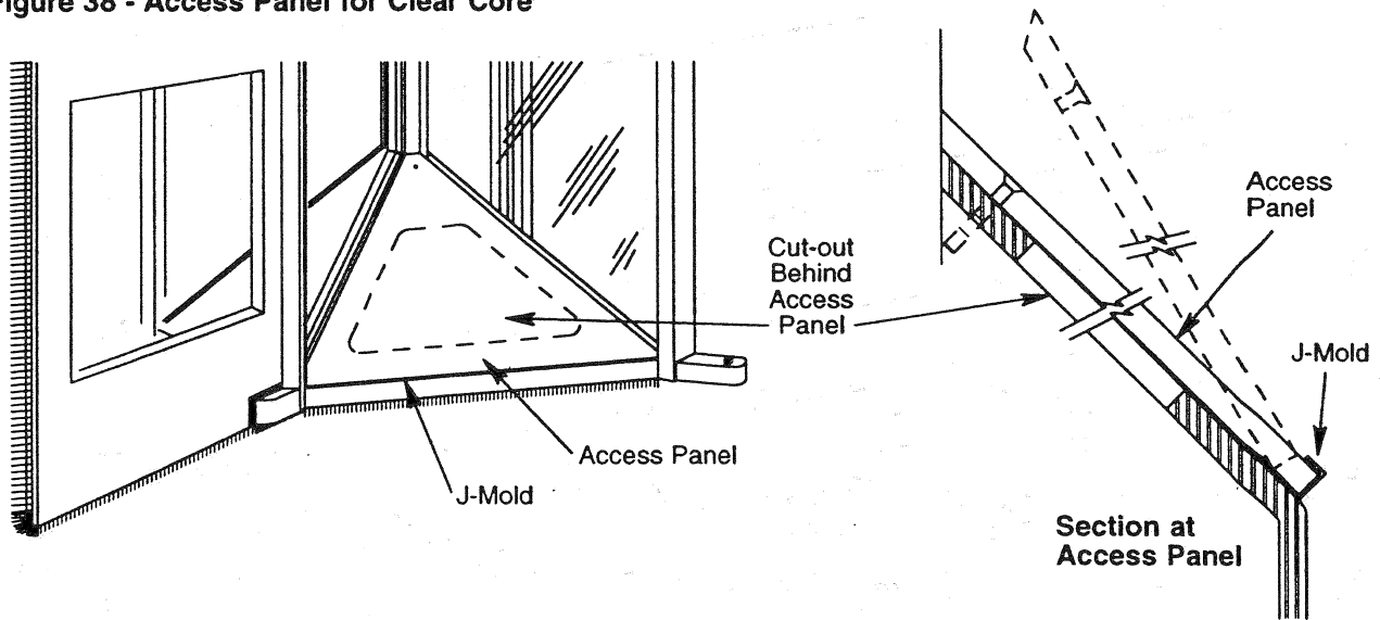
Figure 38 - Access Panel for Clear Core
