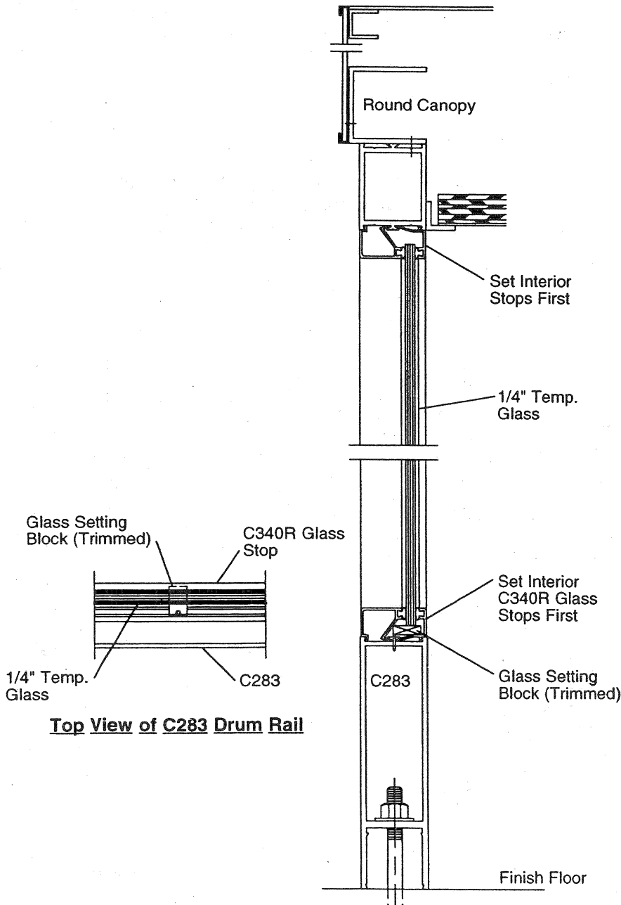
Figure 51 - Segmented Drum Section
