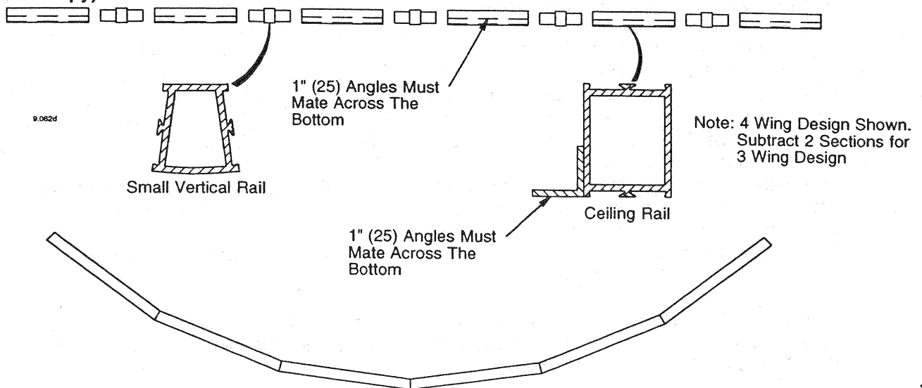
Figure 9- Center Canopy Section Assembly (Round Canopy)
