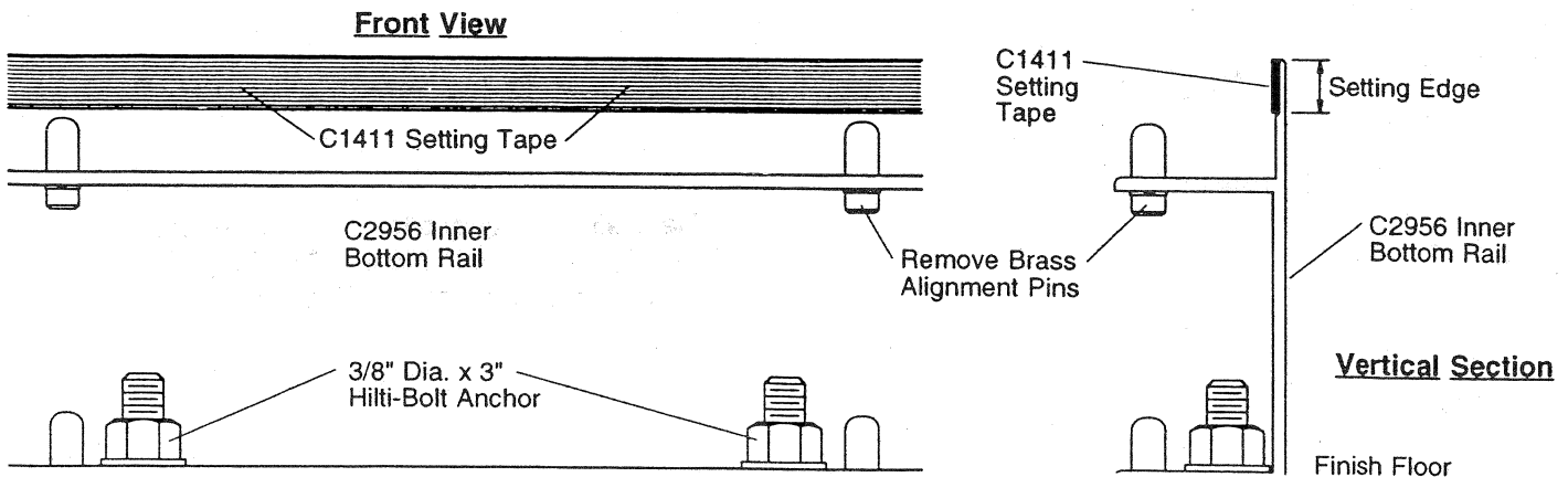
Figure 55 - Inner Bottom Rail
