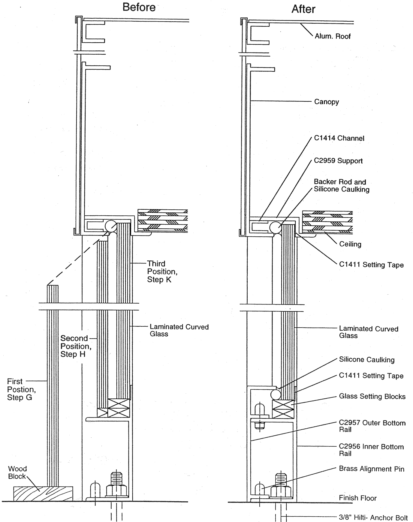
Figure 60 - Vertical Sections
