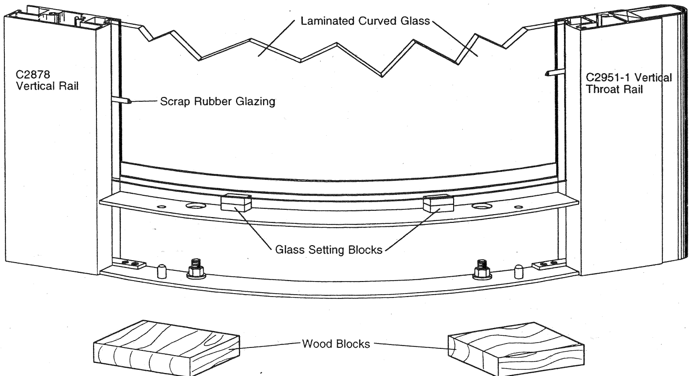
Figure 59 - Bottom View of Enclosure Wall
