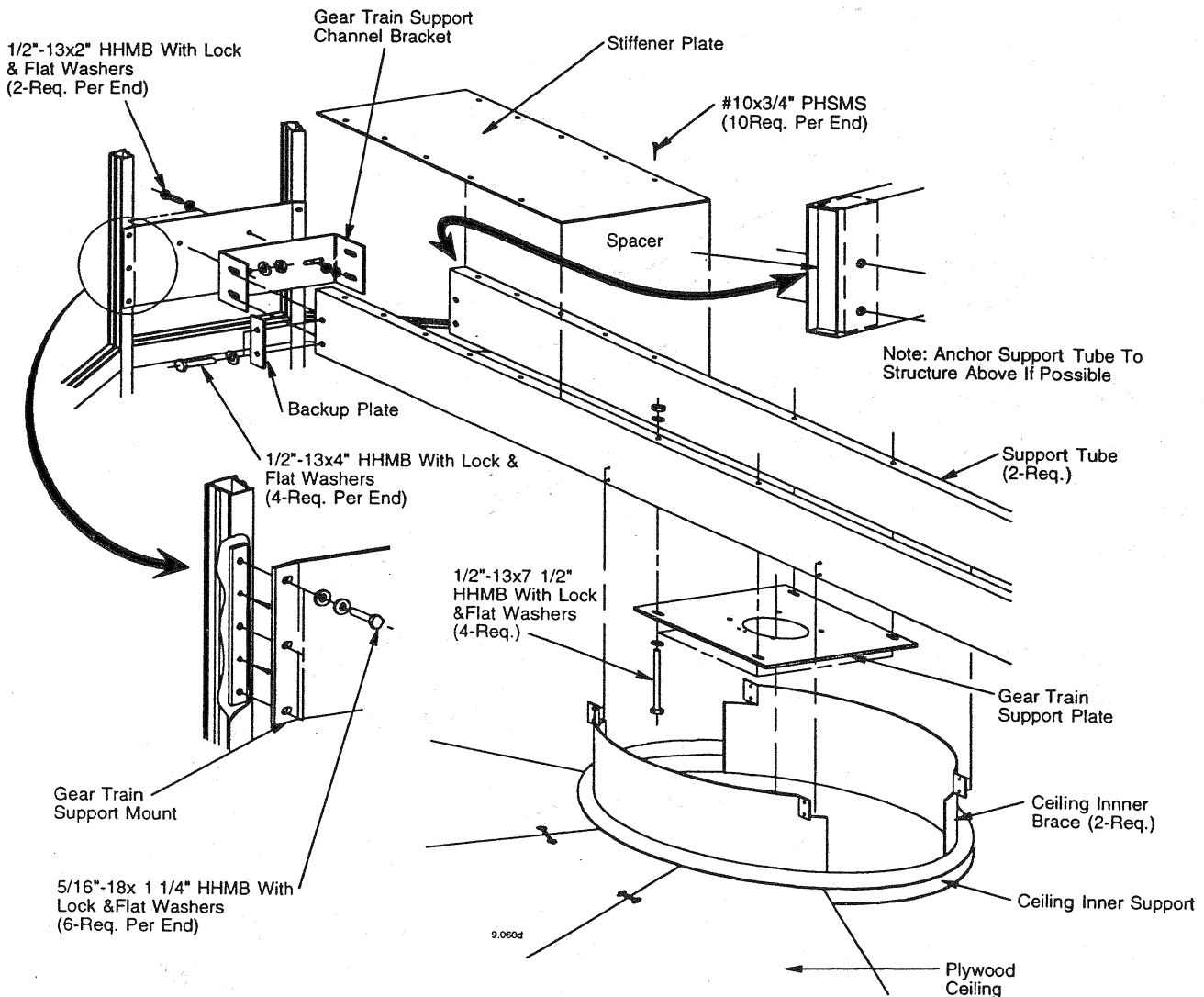
Figure 21 - Gear Train Support (Segmented Canopy)
