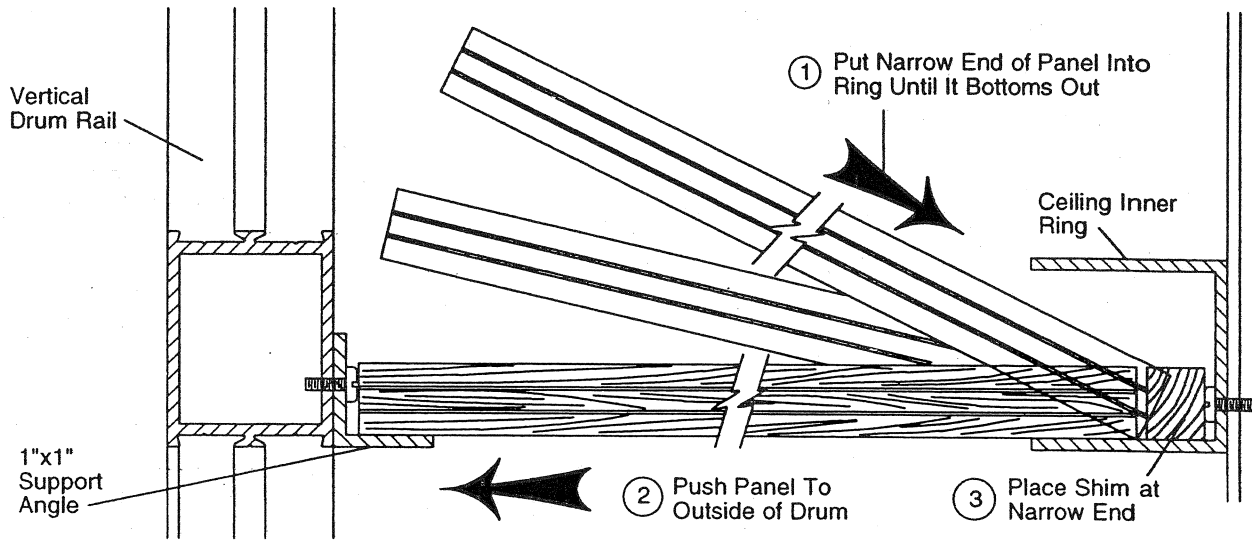
Figure 36 - Ceiling Panel Installation
