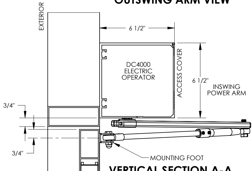
VERTICAL SECTION A-A INSWING ARM VIEW
