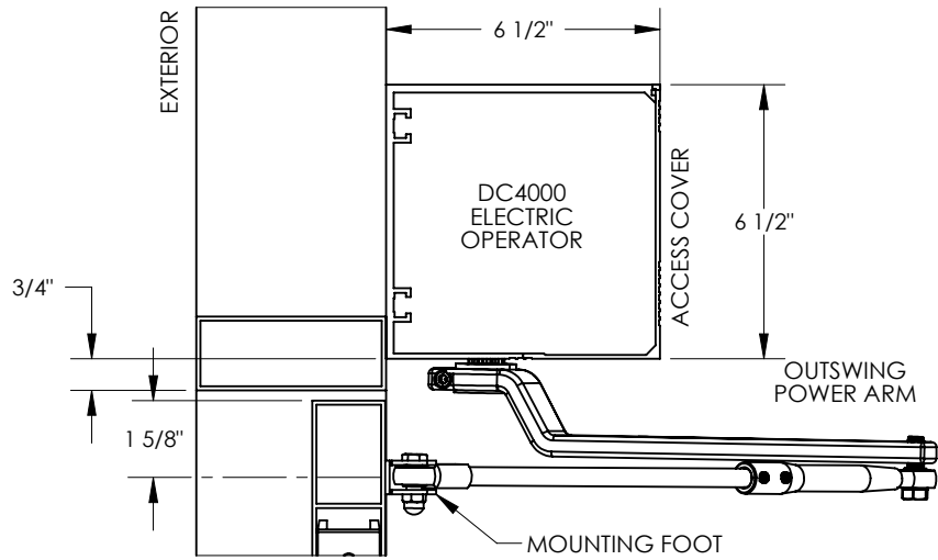
VERTICAL SECTION A-A OUTSWING ARM VIEW
