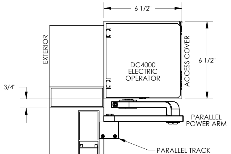
VERTICAL SECTION A-A PARALLEL ARM VIEW
