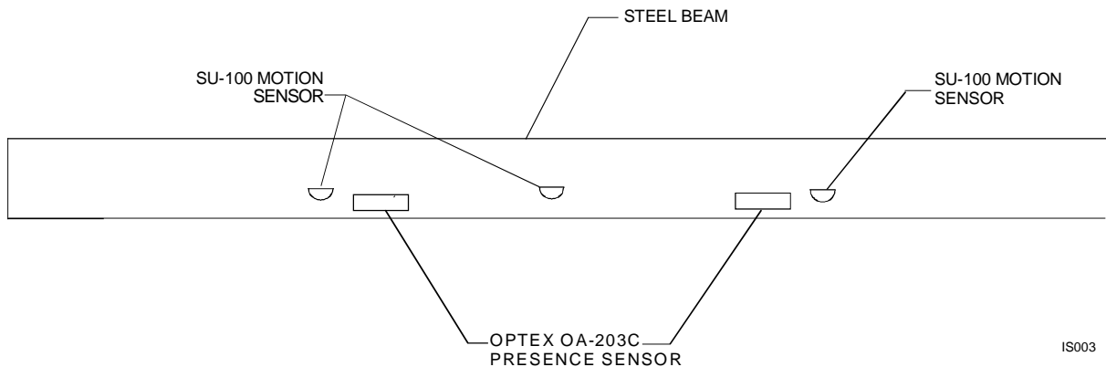
Figure 6. Mounting the Sensors on the Non-Header Side
