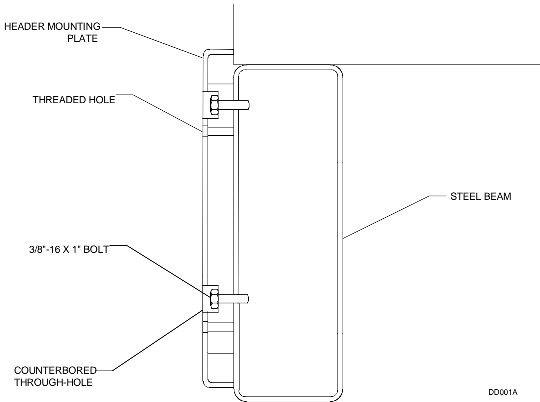
Figure 2. Installing the Header Mounting Plate
