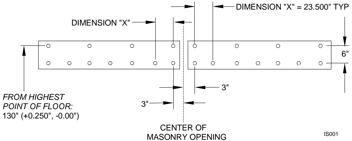
Figure 1. Hole Locations for the Header Mounting Plate
