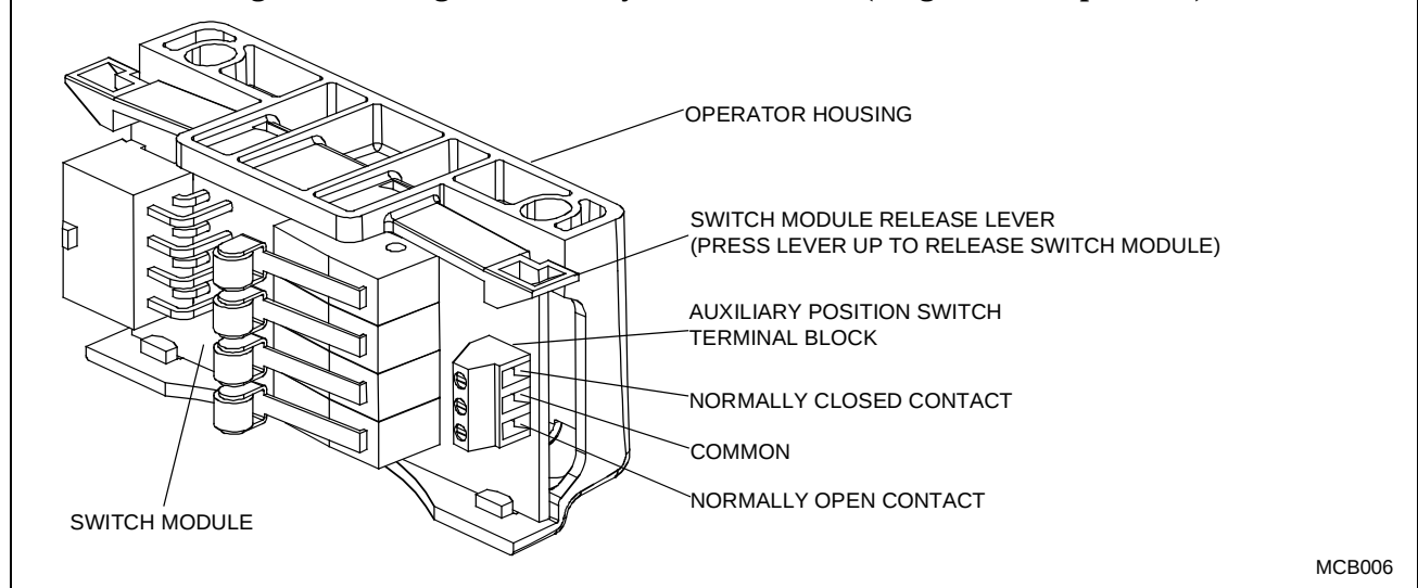
Figure 3. Wiring the Auxiliary Position Switch (Magic-Force Operators)
