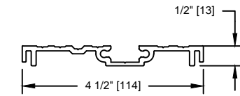
RECESSED BOTTOM TRACK DE0209-01_
