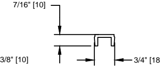
TRACK FILLER DE0196-03_
