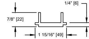
"DRS" SADDLE DE2174-010
