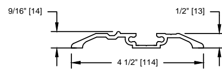
BOTTOM TRACK DE0195-03_
